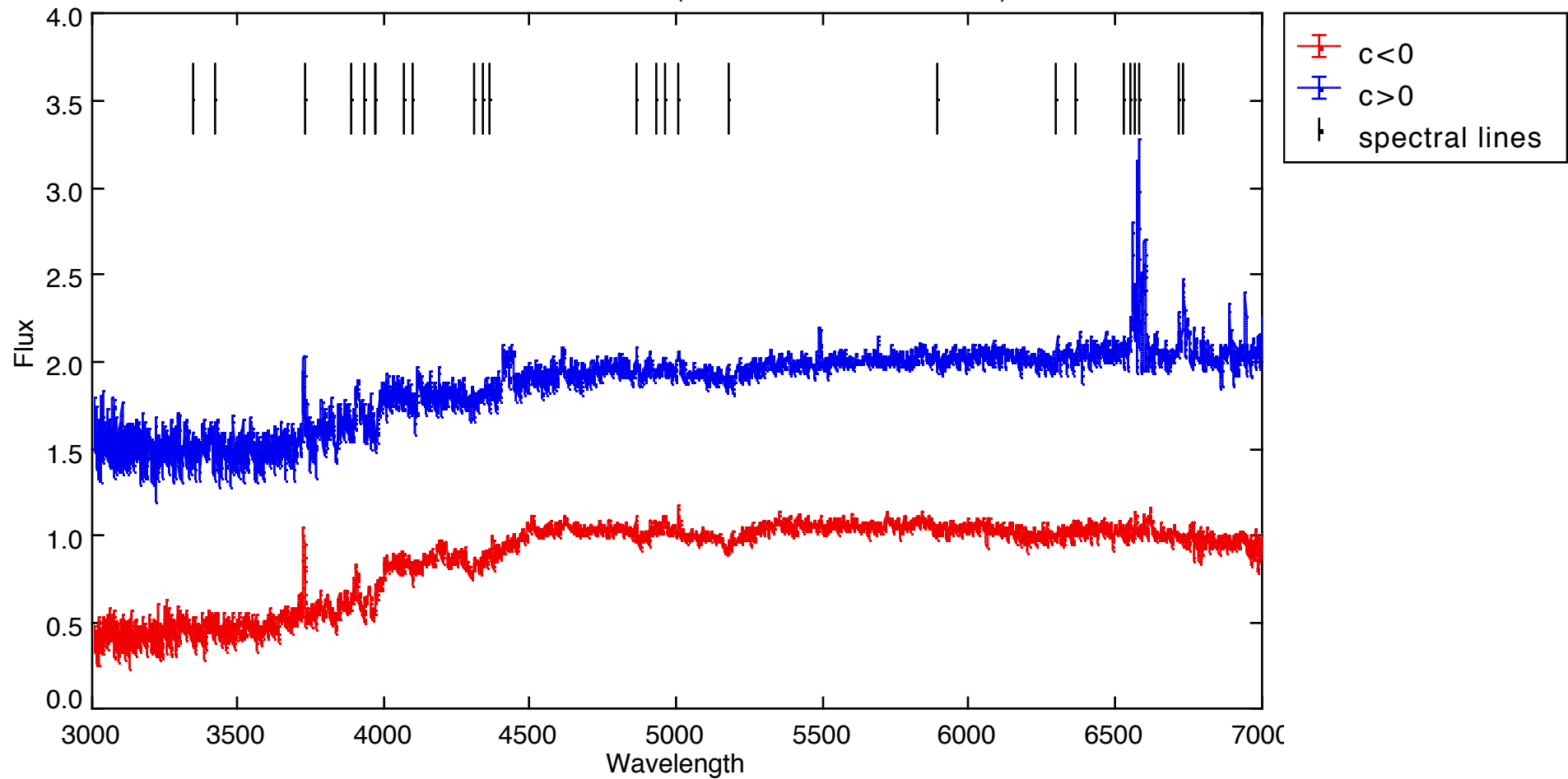
OzDES (Stacks on SNe Ia colour)
